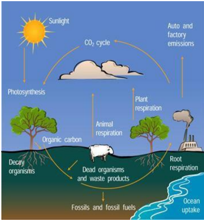
CARBON CYCLE
