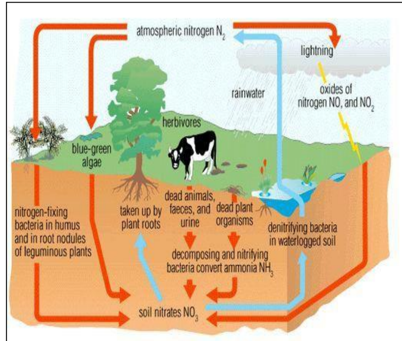
NITROGEN CYCLE
